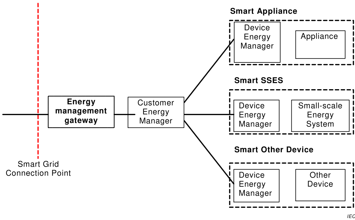
Figure 1 – Logical Architecture
