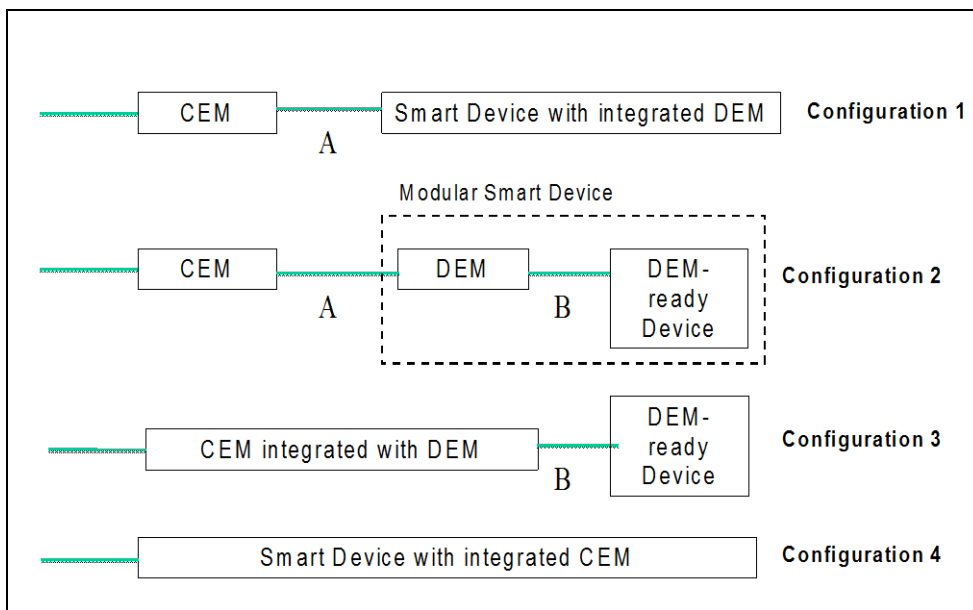
Figure 1 – Logical Architecture
